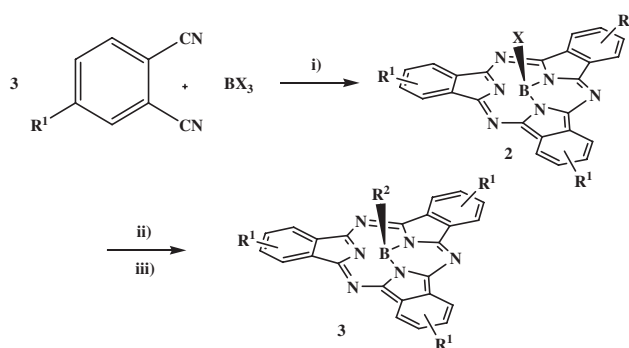
Scheme 2. Synthetic procedure for 3 : i) xylene, reflux; ii) R^2\text{--MgX'}/\text{THF} , -10\text{--}-15\text{ }^\circ\text{C} ; iii) mesitylene, rt.
