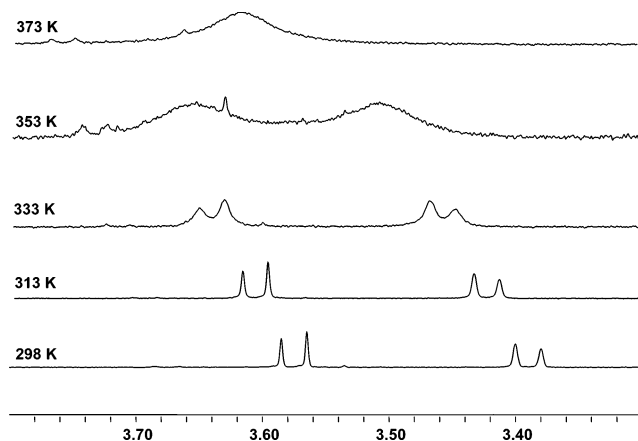
Figure 4. Variable-temperature 1 H NMR spectra of [Cp*ZrL²Me₂].
