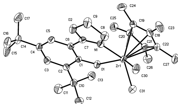
Figure 3. Molecular structure of [Cp*ZrL¹Me₂].
