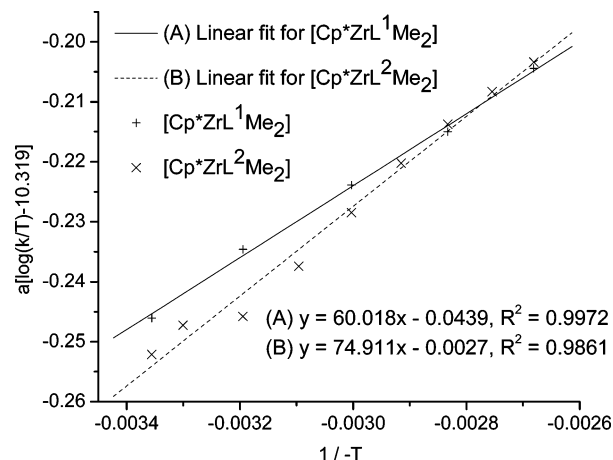
Figure 5. Eyring plot for [Cp*ZrL²Me₂].
