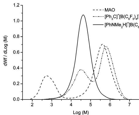
Figure 6. GPC data for PE from [\text{Cp}^*\text{ZrL}^1\text{Cl}_2] and various activators.
