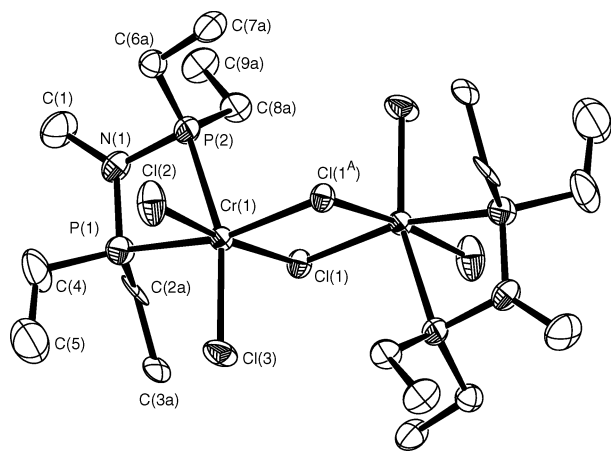
Figure 1. Molecular structure of complex 5. Selected bond distances (Å) and angles (deg): Cr(1)–P(1) 2.4152(13); Cr(1)–P(2) 2.4775(15); Cr(1)–Cl(1) 2.3741(13); Cr(1)–Cl(1A) 2.4191(12); Cr(1)–Cl(2) 2.2839(14); Cr(1)–Cl(3) 2.3168(13); P(1)–N(1)–P(2) 106.32(19); P(1)–Cr(1)–Cl(1) 94.28(5); P(1)–Cr(1)–Cl(2) 88.43(5); P(2)–Cr(1)–Cl(1A) 99.11(5).
