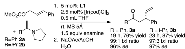
Figure 1. Phosphoramidite ligand L1 and structure of cyclometalated five-coordinate Ir catalyst precursor Ir(cod)(κ 2 - L1 )( L1 ) (5) .
