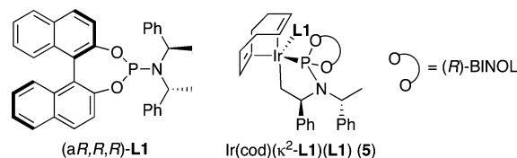
Figure 1. Phosphoramidite ligand L1 and structure of cyclometalated five-coordinate Ir catalyst precursor Ir(cod)(κ 2 - L1 )( L1 ) (5) .
