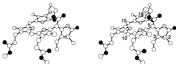
Figure 2. Stereoscopic view of 3'' (R 1 = R 2 = Me, R 3 , R 4 = CHMe, R 5 = CO 2 t Bu, R 6 = Me).
