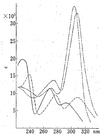
Fig. 2. UV Spectra of Some Typical Derivatives of Isothiazolo[3,4-d]pyrimidine (Solvent: EtOH for IIIa, IVa; 10% Methylcellosolve in EtOH for IIIa, Va)
