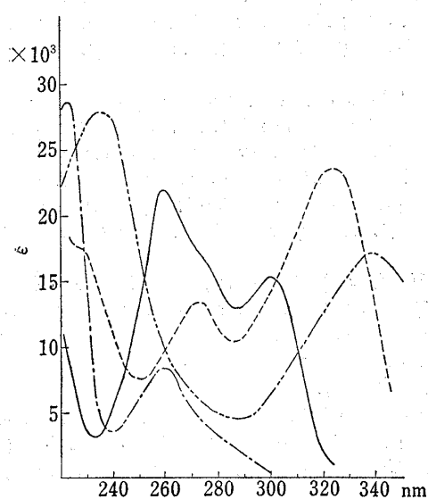
Fig. 1. UV Spectra of Some Typical Derivatives of Pyrimidine (Solvent: EtOH for IIa, VIIa; 10% Methylcellosolve in EtOH for IIa, VIIa)
