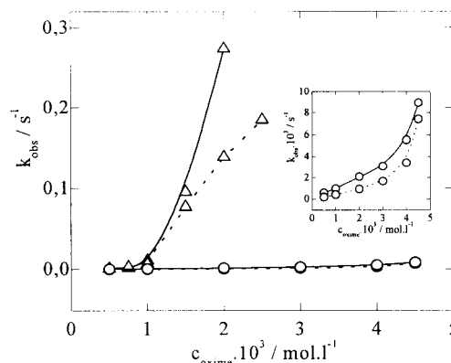
Figure 1. The concentration - rate profile for the PNPP (—) and the PNPH (----) hydrolysis catalyzed by 1a (O) and 1b (Δ). Conditions: [substrate] = 2.0 \times 10^{-5} M, t = 25.0 °C, pH 7.2 (HEPES buffer 0.05 M).
