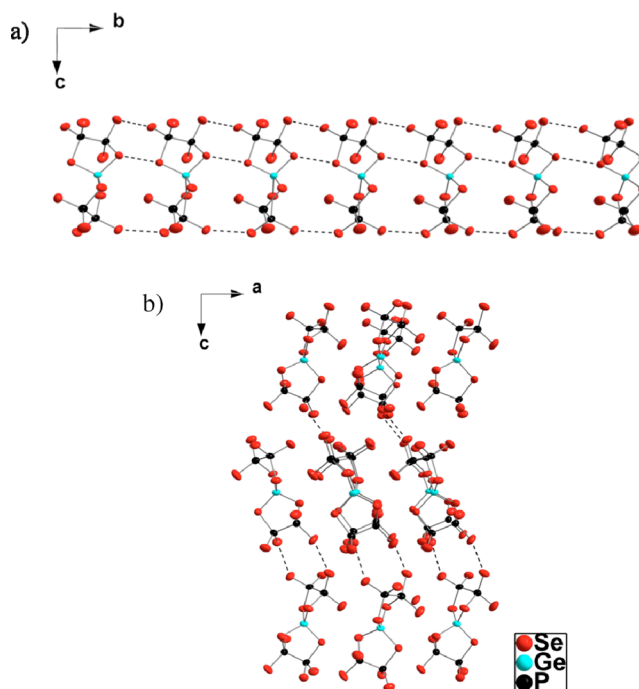
Figure 3. Intermolecular Se...Se interactions shown as dotted lines (a) along the b -axis forming a pseudo one-dimensional chain and (b) along the c -axis, with thermal ellipsoids set at 90%. K cations have been omitted for clarity. Color code: Ge, light blue; P, black; Se, red.
