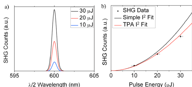
Figure 10. (a) SHG counts for 10, 20, and 30 \mu\text{J} excitation pulse energies for crystalline \text{K}_4\text{GeP}_4\text{Se}_{12} at \lambda = 1200 nm. (b) The corresponding power-dependence plot. The black curve is the predicted power dependence of the SHG when two-photon absorption is absent. The red curve is a fit to the SHG power dependence with \beta = 30.7 cm/GW.
