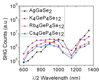
Figure 12. Broadband SHG responses of \text{AgGaSe}_2 (▼), \text{K}_4\text{GeP}_4\text{Se}_{12} (■), \text{Rb}_4\text{GeP}_4\text{Se}_{12} (●), and \text{Cs}_4\text{GeP}_4\text{Se}_{12} (▲) from \lambda = 1200 – 2700 nm.
