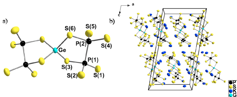
Figure 4. Discrete anionic unit (a) and extended unit cell viewed down the b -axis (b) of K_4GeP_4S_{12} with thermal ellipsoids set at 70%. Color code: K, dark blue; Ge, light blue; P, black; S, yellow.
