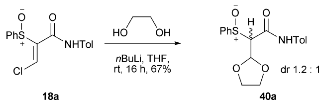
Scheme 20
