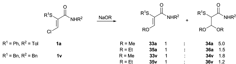
Scheme 18
