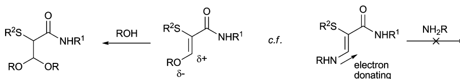
Scheme 17
