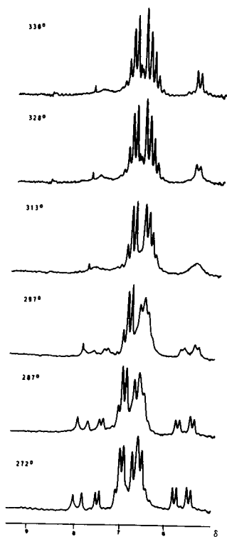
Figure 1. 90 MHz nmr spectra of 1-methyl-4-phenylhydrazino-2-pyrimidone ( 3 ) in 1:1 deuteriodimethylsulfoxide:deuteriochloroform.
