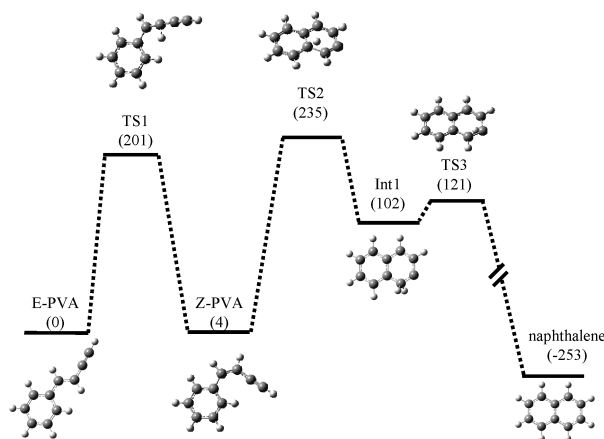
Figure 11. Ground-state potential energy surface for the isomerization from E -PVA and Z -PVA to naphthalene (kJ/mol) calculated employing the B3LYP function using the 6-311+G(d,p) basis set.
