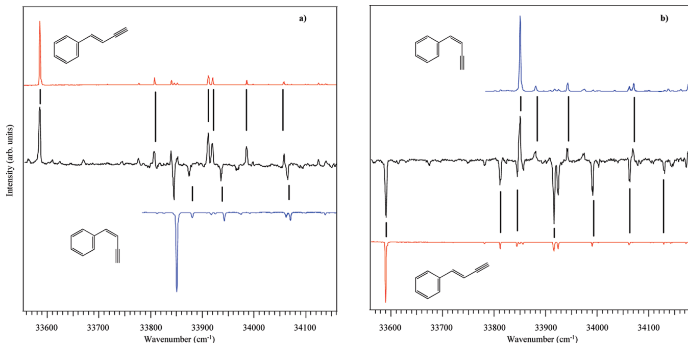
Figure 7. Comparison of LIF spectra (red and blue traces) with hole-filling spectra (red trace) for the (a) Z → E and (b) E → Z isomerizations. In both panels, the middle spectrum is the UV hole-filling spectrum in which population gain produces an increase in signal and population loss a depletion in signal. The LIF spectrum of the depleted species (blue trace) has been inverted for easier comparison.
