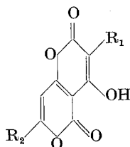
VIII \text{R}_1 = \text{CH}_2\text{C}_6\text{H}_5 , \text{R}_2 = \text{C}_6\text{H}_5 IX \text{R}_1 = \text{H} , \text{R}_2 = \text{C}_6\text{H}_5 X \text{R}_1 = \text{CH}_2\text{C}_6\text{H}_5 , \text{R}_2 = \text{CH}_3
