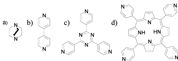
Scheme 1 Templates used in the disulfide porphyrin library: (a) 1,4-diazabicyclo(2.2.2)octane (DABCO), (b) 4,4'-bipyridine (Bipy), (c) 4-s-tripyril triazine (TPyT), (d) tetrapyrilporphyrin (TPyP).
