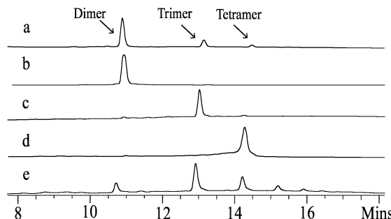
Fig. 3 HPLC traces of the porphyrin DCL in the a) absence of a template, b) presence of DABCO, c) presence of TPyT, d) presence of TPyP, and e) presence of Bipy.
