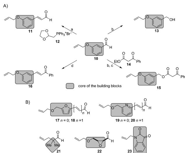
Scheme 2. Building blocks. A) Diversification of aldehyde 10 toward “alophile” components. B) Building blocks with different cores. Reaction conditions: a) 12 (3 equiv), NaOMe, DMF/MeOH 2:1, reflux, 55 %; b) NaBH 4 , NaHSO 4 , H 2 O, CH 3 CN, 81 %; c) 14 (1 equiv), 4-NO 2 -C 6 H 4 -B(OH) 2 (2.5 mol %), toluene, 79 %; d) acetophenone, EtOH/SOCl 2 10:1, 99 %. DMF = N,N -dimethylformamide.
