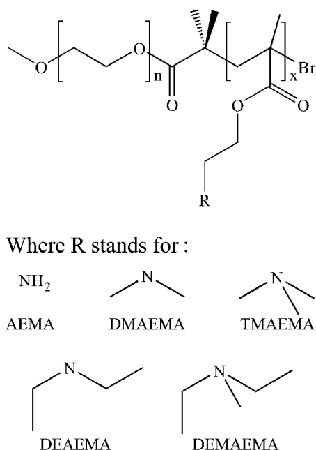
Fig. 1. Structure of the amino diblock copolymers studied.
