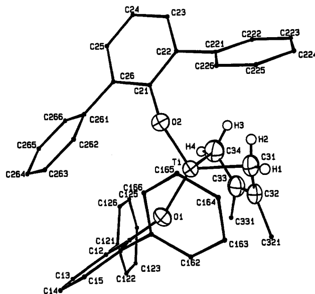
Figure 1. ORTEP view of the titanacycle compound 1. Selected bond distances (Å) and angles (deg): Ti-O(1) = 1.804 (2); Ti-O(2) = 1.843 (2); Ti-C(31) = 2.096 (4); Ti-C(32) = 2.299 (3); Ti-C(33) = 2.290 (4); Ti-C(34) = 2.109 (5); C(31)-C(32) = 1.436 (5); C(32)-C(33) = 1.384 (6); C(33)-C(34) = 1.442 (6); O(1)-Ti-O(2) = 115.2 (1); C(31)-Ti-C(34) = 87.0 (1); Ti-O(1)-C(11) = 151.2 (1); Ti-O(2)-C(21) = 143.6 (2).
