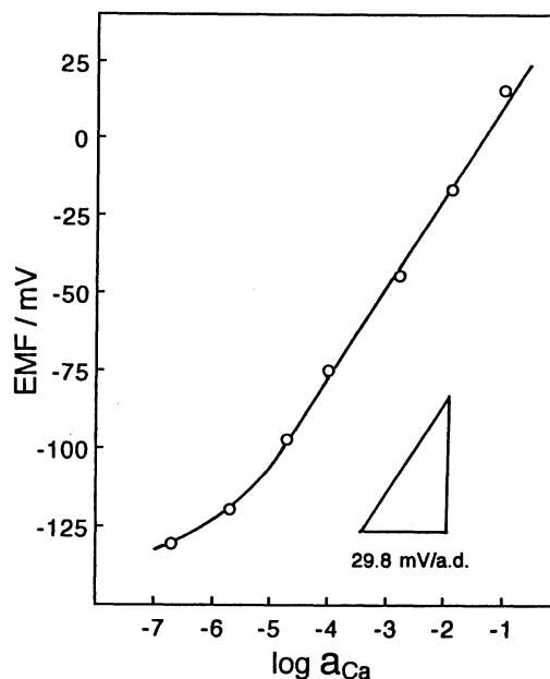
Fig. 4. Response of the membrane electrode based on 1 toward the \text{Ca}^{2+} activity.
