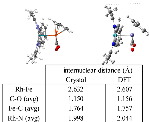
Figure 6. ORTEP representation of (\text{tmtaa})\text{Rh}-\text{FeCp}(\text{CO})_2 ( 9 ) structure from single crystal X-ray diffraction with thermal ellipsoids shown on non-hydrogen atoms at 50% probability level, hydrogen atoms shown as open circles, and energy minimization by DFT computations (B3LYP, 3-21G/6-31G*). A table of selected internuclear distances observed in the molecular structure and calculated by DFT is also included.
