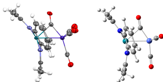
Figure 7. Drawing of the semibridging carbonyl in (tmtaa)Rh-Co(μ-CO)(CO) 3 showing the donation of rhodium dπ into the C≡O π* orbital.
