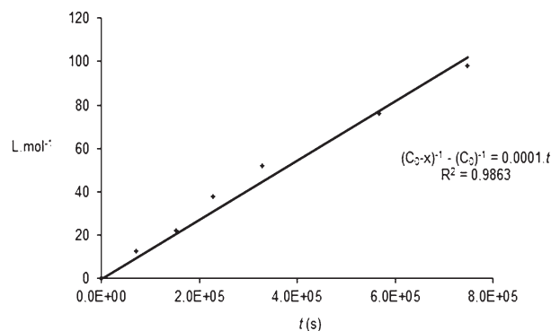
Figure 4. Example of determination of second-order rate constants for the reaction of azetidinium salts 8 with 4-DMAP in \text{CD}_3\text{CN} (20 °C) by NMR. [\text{DMAP}]_0 = [\text{8}]_0 = 1.60 \times 10^{-3} \text{ mol} \cdot \text{L}^{-1} . k = 1.4 \times 10^{-4} \text{ L} \cdot \text{mol}^{-1} \cdot \text{s}^{-1} .
