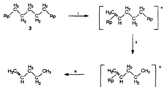
Scheme 2. \text{Rp} = \text{CpRu}(\text{CO})_2 for the following reagents and conditions: (i) [\text{Ph}_3\text{C}][\text{PF}_6] ; (ii) \text{CF}_3\text{COOH} ; (iii) \text{NaI} , acetone.
