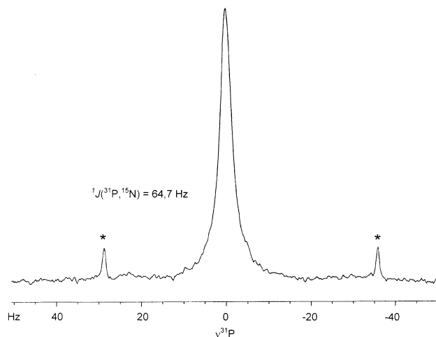
Fig. 1. 103.1 MHz ^{31}\text{P} -NMR spectrum of \text{fc}[\text{P}-\text{N}^i\text{Pr}_2] ( 1 ) in \text{C}_6\text{D}_6 , recorded by using the HEED-INEPT pulse sequence with ^1\text{H} decoupling [15] (Hahn-echo delay of 0.18 s; result of 200 transients, spectrometer time 8 min). The ^{15}\text{N} satellites are marked by asterisks ( ^1\Delta^{14/15}\text{N}(^{31}\text{P}) = -35.0 \pm 1 ppb).
