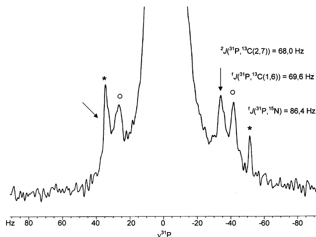
Fig. 2. 202.5 MHz ^{31}\text{P}\{^1\text{H}\} -NMR spectrum of 1 showing the parent line together with ^{13}\text{C} and ^{15}\text{N} satellites (2716 transients; 2 h of spectrometer time). Note that the ^{15}\text{N} satellites (marked by asterisks; ^1\Delta^{14/15}\text{N}(^{31}\text{P}) = -39 \pm 2 ppb) are much sharper than the ^{13}\text{C} satellites for ^1J(^{31}\text{P}, ^{13}\text{C}(1,6)) (marked by open circles; ^1\Delta^{12/13}\text{C}(^{31}\text{P}) = -36 \pm 2 ppb) and ^2J(^{31}\text{P}, ^{13}\text{C}(2,7)) (marked by arrows; ^2\Delta^{12/13}\text{C}(^{31}\text{P}) < 2 ppb).
