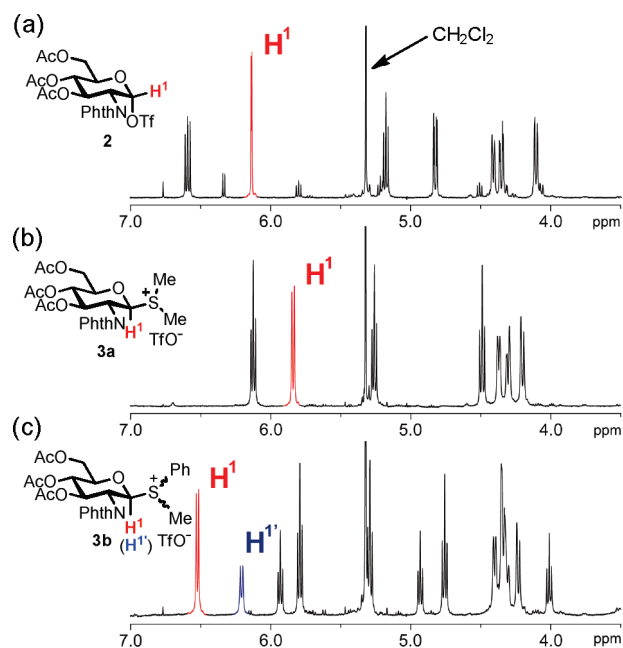
Figure 1. ^1\text{H} NMR spectra at -80^\circ\text{C} : (a) glycosyl triflate 2 , (b) glycosyl sulfonium ion 3a , and (c) glycosyl sulfonium ion 3b .
