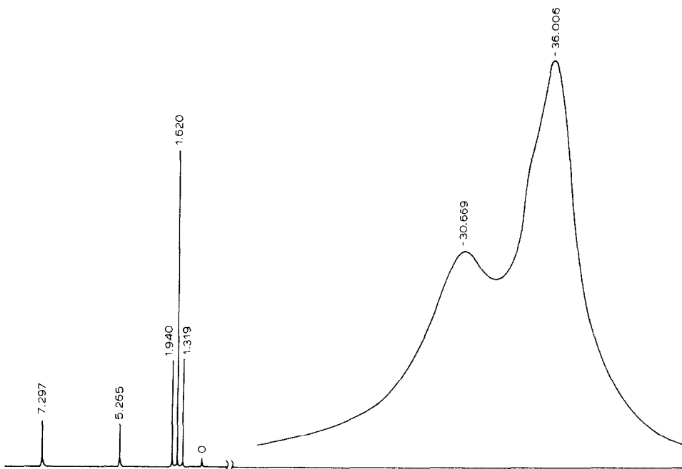
Fig. 1. 1 H NMR spectrum of IV \cdot \text{OCOCF}_3 after partial conversion into V \cdot (\text{OCOCF}_3)_2 .
