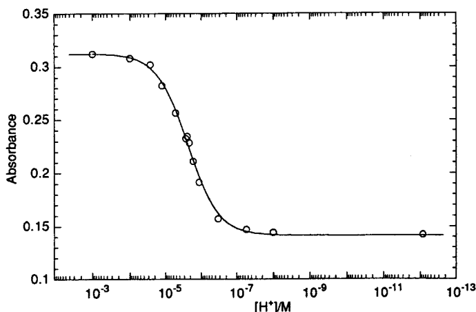
Figure 1. Spectrophotometric titration curve for the ionization of (Z)-β-methoxymethacrylic acid in aqueous solution at 25 °C
