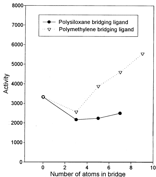
Fig. 1. Variation of activity (kg PE/mol Zr h atm) with the number of atm in bridging ligand. For number of atoms in the bridge = 0, catalyst = (\text{Cp})(\text{ind})\text{ZrCl}_2 . For number of atoms in the bridge = 3, ( \nabla ) complex 10, ( \bullet ) [\text{O}(\text{SiMe}_2\text{C}_5\text{H}_4)_2][(\text{C}_9\text{H}_7)\text{ZrCl}_2]_2 . For number of atoms in the bridge = 5, ( \nabla ) complex 11, ( \bullet ) [\text{O}(\text{SiMe}_2\text{C}_5\text{H}_4)_2][(\text{C}_9\text{H}_7)\text{ZrCl}_2]_2 . For number of atoms in the bridge = 7, ( \nabla ) complex 12, ( \bullet ) [\text{O}\{\text{O}(\text{SiMe}_2)_2\text{C}_5\text{H}_4\}_2][(\text{C}_9\text{H}_7)\text{ZrCl}_2]_2 . For number of atoms in the bridge = 9, ( \nabla ) complex 13.
