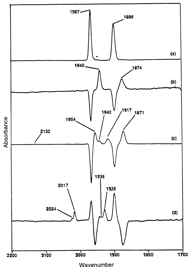
Fig. 5. IR spectra of \text{Mo(CO)}_2[\eta^5, \eta^3\text{-C}_5\text{H}_4\text{-C(CH}_3)_2\text{-C}_5\text{H}_6] ( I ). (a) Starting material. (b) Subtraction spectrum, 120 min irradiation \lambda = 500 \pm 70 nm minus (a). (c) Subtraction spectrum, 30 min irradiation at 350 < \lambda < 370 nm minus (a). (d) Subtraction spectrum, anneal to 173 K minus 120 min photolysis at 350 < \lambda < 370 nm. * This band arises from a natural abundance of ^{13}\text{CO} .
