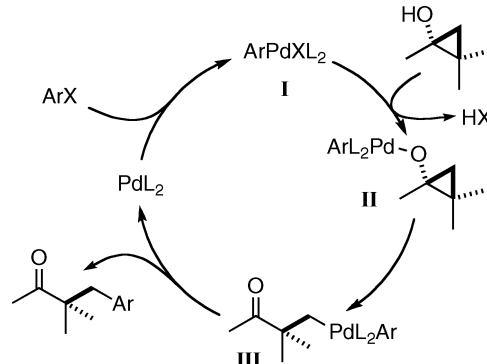
Scheme 1. Proposed Catalytic Cycle for the Cross-Coupling of Palladium Homo-enolates with Aryl Halides
