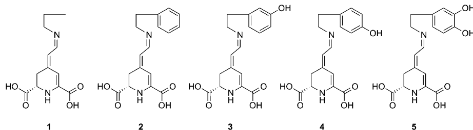
Figure 1. Structures for the betalainthins. Structures 4 and 5 correspond to naturally occurring miraxanthins III and V, respectively. Compound 2 has been found on certain cacti, and compounds 1 and 3 are novel pigments.
