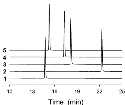
Figure 2. HPLC chromatographic profiles for individual pigment analysis of purified samples. A 20 \mu L amount of pure pigment solutions was injected with a concentration of 50 \mu M. Absorbance was detected at \lambda = 480 nm. Full scale is 0.2 absorbance units.
