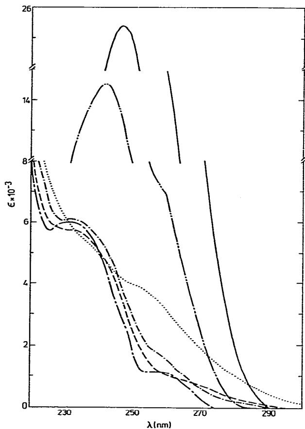
Fig. 2. Ultraviolet absorption spectra of substituted methylocyclohexasilanes RR'Si(Me_2Si)_5 : R, R' = Me , Me (1b), ———; Me, Cl (2b), ———; Me, Ph (3b) ———; Ph, Ph (4b), ———; Me, t-Bu (5b), ———; t-Bu, t-Bu (6b), ·····.
