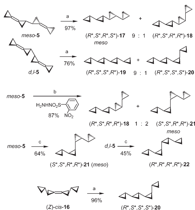
Scheme 3. Reduction of bis(bicyclopropylidenyl)s meso -5 and d,l -5, as well as of ( Z )- cis -16 under various conditions. a) Li, liq. NH 3 , −78°C, 1.5 h, then MeOH, −78→20°C; b) 2-nitrobenzenesulfonyl hydrazide (8.7 equiv), MeOH, 20°C, 5 h; c) H 2 , Pd/BaSO 4 (2 mol %), MeOH, 20°C, 16–44 h.
