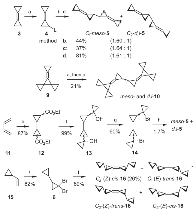
Scheme 2. Preparation of the diastereomeric bis(bicyclopropylylidenyl)s meso - 5 and d,l - 5 as well as meso - 10 and d,l - 10 under various conditions and as cupric chloride-assisted dehalogenative dimerization of 1,1-dibromo-2-cyclopropylcyclopropane ( 6 ). a) n BuLi, THF, 0^{\circ}\text{C} , 1 h; b) \text{MgBr}_2 , \text{Et}_2\text{O} , -78 \rightarrow 20^{\circ}\text{C} , 1 h, then \text{CuCl}_2 , -78 \rightarrow 20^{\circ}\text{C} , 2.5 h; c) \text{CuCN} , -100 \rightarrow -40^{\circ}\text{C} , 0.5 h, then \text{O}_2 , -78^{\circ}\text{C} , 0.5 h; d) [\text{CuIBu}_3\text{P}]_4 , -78^{\circ}\text{C} , 1 h, then \text{O}_2 , -78^{\circ}\text{C} , 1 h; e) \text{N}_2\text{CHCO}_2\text{Et} , [\text{Rh}(\text{OAc})_2]_2 (0.3 mol %), \text{CH}_2\text{Cl}_2 , -5 \rightarrow 0^{\circ}\text{C} , 12.5 h; f) \text{EtMgBr} , \text{Ti}(\text{O}i\text{Pr})_4 , \text{Et}_2\text{O} , 20^{\circ}\text{C} ; g) \text{Ph}_3\text{P-Br}_2 , \text{Py} , \text{CH}_2\text{Cl}_2 , -30 \rightarrow 20^{\circ}\text{C} , 24 h; h) t BuOK, DMSO, 20^{\circ}\text{C} , 24 h; i) \text{CHBr}_3 , KOH (pellets), TEBACl, \text{CH}_2\text{Cl}_2 , 20 \rightarrow 25^{\circ}\text{C} , 2 h; j) \text{CuCl}_2 , THF, -100^{\circ}\text{C} , slow addition of n BuLi over 1 h, then -100 \rightarrow 20^{\circ}\text{C} , 2 h.
