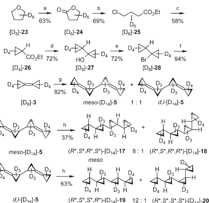
Scheme 4. Preparation of meso -[D 14 ]-5 and d,l -[D 14 ]-5 per-deuteriobis(bicyclopropylidenyl)s as well as their Birch reduction. a) Ca(OC 2 H 5 ) 2 (2 equiv), MeCN/AcOH (3:2), 0→20°C, 22 h; b) SOCl 2 , 80°C, 3 h, then EtOH, 20→78°C, 1.5 h at 78°C; c) EtONa, EtOH, 20→78°C, 1 h at 78°C, then aq. 10 M H 2 SO 4 , 0°C; d) C 2 D 5 MgBr, Ti(O i Pr) 4 , Et 2 O, 20°C, 1 h, then aq. 10% H 2 SO 4 , 0°C, 1 h; e) Ph 3 P-Br 2 , Py, CH 2 Cl 2 , −15→20°C, 48 h; f) n BuOK, DMSO, 20°C, 48 h; g) n BuLi, THF, 20°C, 1 h, then CuCN, −100→−40°C, 0.5 h, then O 2 , −78°C, 0.5 h; h) Li, liq. NH 3 , −78°C 1.5 h, then MeOH, −78→20°C.
