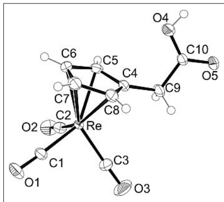
Fig. 2. ORTEP representation of 8 . Relevant bond lengths (Å): Re(1)–C(1) 1.912(2), Re(1)–C(2) 1.917(2), Re(1)–C(3) 1.913(2), Re(1)–C(7) 2.299(2), Re(1)–C(6) 2.3002(19), Re(1)–C(5) 2.301(2), Re(1)–C(4) 2.3053(19), Re(1)–C(8) 2.308(2).
