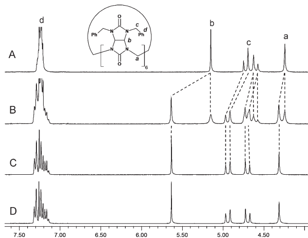
Figure 3. ^1\text{H} NMR spectra (300 MHz, \text{CDCl}_3 ) of Bn 12 BU[6] in the absence (A) and in the presence of 0.5 equiv (B), 1.1 equiv (C), and 2.2 equiv (D) of \text{TBA}^+\text{Cl}^- .
