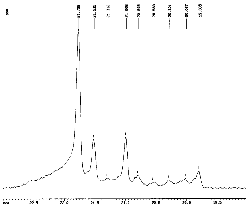
Fig. 3. ^{13}\text{C} NMR spectrum of the methyl pentad region of PP obtained with 1 -MAO at T_p = 50^\circ\text{C} .
