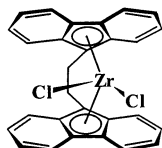
Abb. 1. [1,2-Bis(η 5 -9-fluorenyliden)ethandiylium]zirconiumdichlorid [C 13 H 8-n R n (CH 2 ) 2 C 13 H 8-n R n ][ZrCl 2 ] ( n = 0; R = H).
