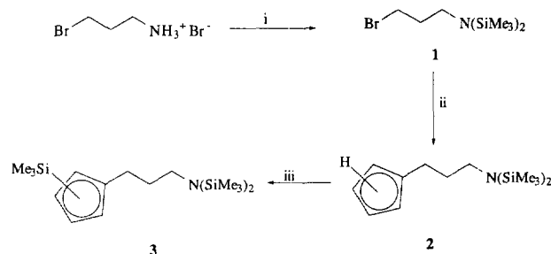
Scheme 1. Synthesis of the ligand precursor 3 . (i) (Me_3Si)SO_3CF_3 (3 equiv.) and NEt_3 (3 equiv.) in Et_2O , 0°C to r.t., 4 h. (ii) Na(C_5H_5) (1.1 equiv.) in THF, -10°C to r.t., 12 h. (iii) t-BuLi (1 equiv.) in hexane, -78°C to r.t., 12 h, then Me_3SiCl (1.5 equiv.) 5 h.
