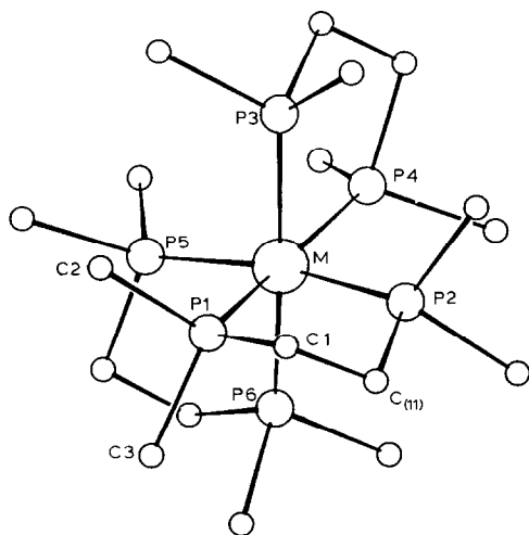
Fig. 4. The molecular structure of \text{M}(\text{Me}_2\text{PCH}_2\text{CH}_2\text{PMe}_2)_3 . The atoms labelled P(2), P(3), P(4), P(5) and P(6) are related to P(1) by the operations y, x, 0 ; \bar{y}, 0, x ; x, 0, y ; 0, \bar{x}, \bar{y} and 0, \bar{y}, \bar{x} respectively and the atom labelled C(11) to that labelled C(1) by the operation y, x, \bar{z} .
