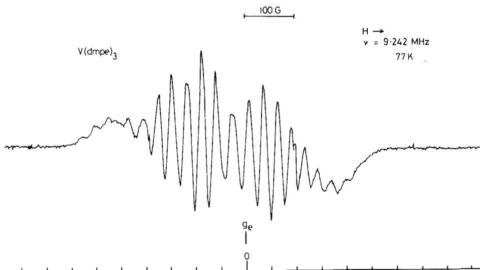
Fig. 2. ESR (9.242 GHz, modulation amplitude 4 G) spectrum of \text{V}(\text{dmpe})_3 at 77 K in frozen toluene.
