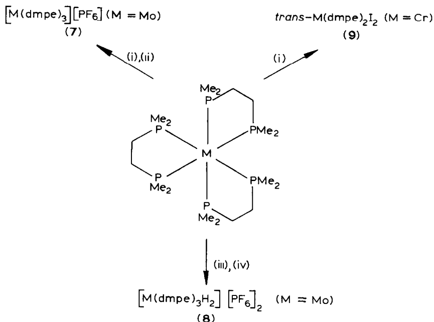
SCHEME 1. (i) M = Cr, Mo, W, V, Nb, Ta , yields ca. 55%. (ii) Methyl iodide in toluene at room temperature, 88%. (iii) HCl gas, 5 min then NH_4PF_6 aq., > 90%. (iv) Methyl iodide in toluene, 85%.
