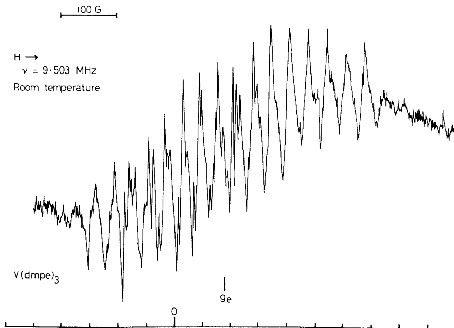
Fig. 1. ESR (9.504 GHz, modulation amplitude 8 G) spectrum of V(dmpe)_3 at room temperature in toluene (maximum gain).
