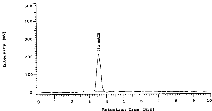
Figure 3. HPLC radiochromatogram from the analysis (Analysis programme 2) of a plasma sample taken 30 min after i.v. administration of [N-methyl- ^{11}\text{C} ]Me-AIB to humans.
