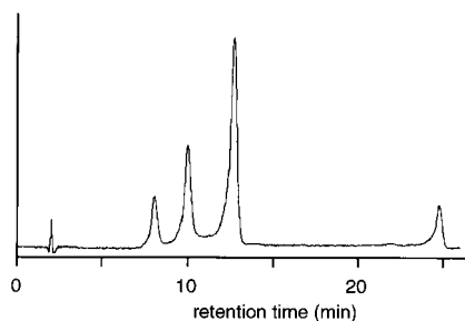
Figure 1. HPLC analysis of a mixture of atropisomers 1 at equilibrium. YMC-packed column AQ-312 (reversed phase); eluent, MeOH/ iso -PrOH = 65:35–20:80 (1 mL min −1 ), monitored by UV/vis spectroscopy (420 nm). The relative amounts of the four atropisomers and the respective retention times are as follows: 1 aaaa , 10.5% (24.8 min); 1 aaab , 54.0% (12.6 min); 1 abab , 24.0% (10.0 min); 1 abba , 11.6% (7.95 min).
