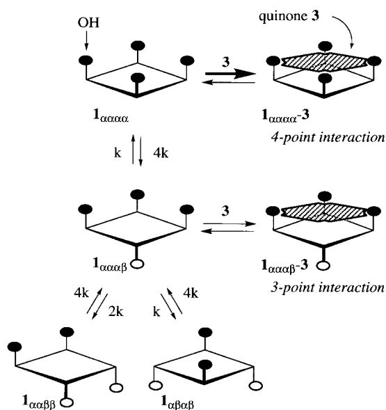
Scheme 5. Proposed mechanism of induced-fit molecular recognition between porphyrin 1 and tetramethoxy- p -benzoquinone 3 .
