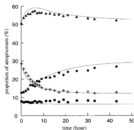
Figure 9. Experimental and simulated results for the atropisomerization of 1 upon addition of 4 . The lines represent the simulation curves calculated from Equations (1)–(6). [\mathbf{1}] = 2.4 mM, [\mathbf{4}] = 7.2 mM in \text{CDCl}_3 at 25^\circ\text{C} . \mathbf{1}_{aaaa} (●), \mathbf{1}_{aaab} (△), \mathbf{1}_{aabb} (+), \mathbf{1}_{abbb} (■).
