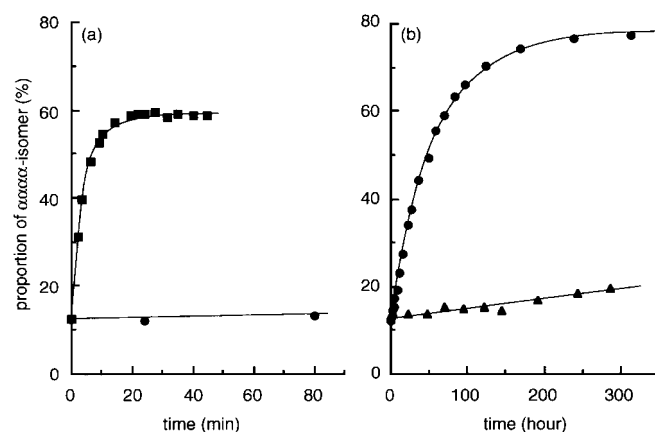
Figure 10. Changes in the relative amounts of atropisomers 1 aaaa · Ni (■), 1 aaaa (●), and 1 aaaa · Zn (▲) with time, upon addition of 3 in CDCl 3 at 25 °C. [ 1 · Ni ] = [ 1 ] = [ 1 · Zn ] = 2.4 mM, [ 3 ] = 7.2 mM.
