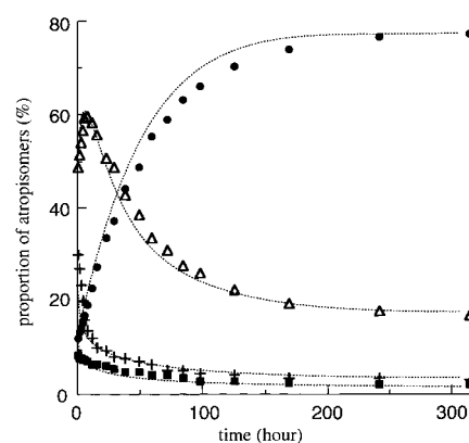
Figure 8. Experimental and simulated results for the atropisomerization of 1 upon addition of 3 . The lines represent the simulation curves calculated from Equations (1)–(6). [\mathbf{1}] = 2.4 mM, [\mathbf{3}] = 7.2 mM in \text{CDCl}_3 at 25^\circ\text{C} . \mathbf{1}_{aaaa} (●), \mathbf{1}_{aaab} (△), \mathbf{1}_{aabb} (+), \mathbf{1}_{abbb} (■).
