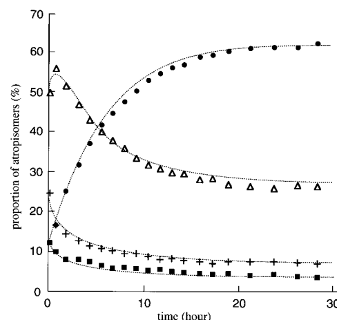
Figure 11. Comparisons of best fits to Equations (1)–(4) with experimental data for the atropisomerization of 1 · Ni upon addition of 3 . [ 1 · Ni ] = 2.4 mM, [ 3 ] = 7.2 mM in CDCl 3 at 25 °C. 1 aaaa · Ni (●), 1 aaaa · Ni (Δ), 1 aaab · Ni (+), 1 abab · Ni (■). Initial isomer contents are 12.5, 50.0, 25.0, and 12.5%, respectively.
