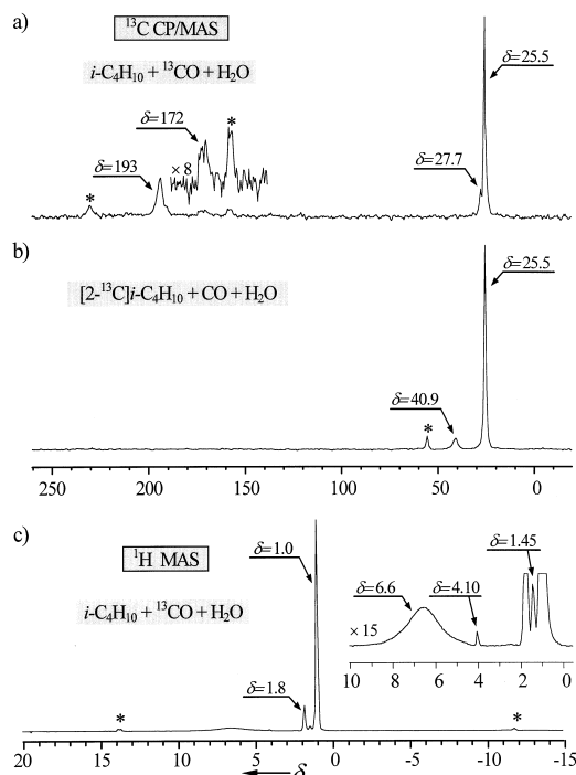
Figure 2. NMR spectra for isobutane, CO, and water coadsorbed on H-ZSM-5 zeolite. The sample was heated at 423 K for 2 h. a) 13 C CP/MAS NMR, coadsorption of unlabeled isobutane, 13 CO (90% 13 C enrichment) and water; b) 13 C CP/MAS NMR, coadsorption of [2- 13 C]isobutane (82% 13 C enrichment), unlabeled CO and water; c) 1 H MAS NMR spectrum of the sample (a). 16000 scans were collected for (a) and (b), 240 scans for (c). Spinning rate was 4.7 kHz for (a), 3.0 kHz for (b), 5.1 kHz for (c). Asterisks (*) in the spectra denote spinning side bands.
