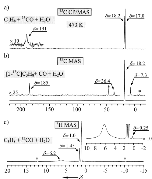
Figure 1. NMR spectra of propane, carbon monoxide, and water coadsorbed on H-ZSM-5 zeolite. The samples were heated at 473 K for 2 h. a) 13 C CP/MAS NMR, coadsorption of propane, 13 CO (90% 13 C enrichment) and water; b) 13 C MAS NMR, coadsorption of [2- 13 C]propane (99% 13 C enrichment), unlabeled CO and water; c) 1 H MAS NMR spectrum of the sample (a). 16 000 scans were collected for (a) and (b), 120 scans for (c). Spinning rate was 4.5 kHz for (a) and (c), 2.7 kHz for (b). Asterisks (*) in the spectra denote spinning side bands.
