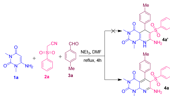
Scheme 1. Three-component reaction of 1,3-dimethyl-6-aminouracil 1a , phenylsulfonyl acetonitrile 2a , and 4-methylbenzaldehyde 3a .
