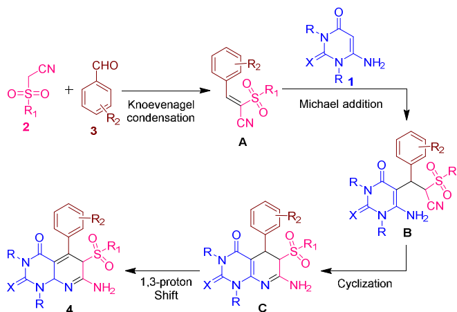
Scheme 2. Plausible mechanism for the formation of 4 .
