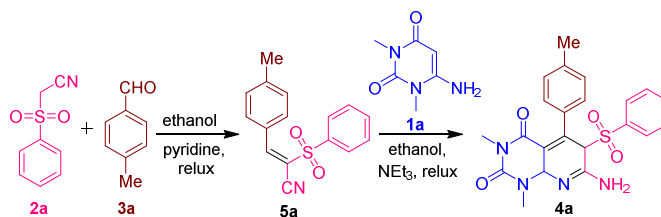
Scheme 3. Stepwise experiments for the synthesis of 4a .
