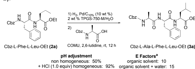
Fig. 2 Importance of pH on the tandem deprotection/coupling sequence for tripeptide synthesis, and E Factor calculations for the 2-step process. a Single run on a 3.5 mmol scale; 20 mL of MTBE were used for extraction, isolated yield: 86% (1.53 g)
