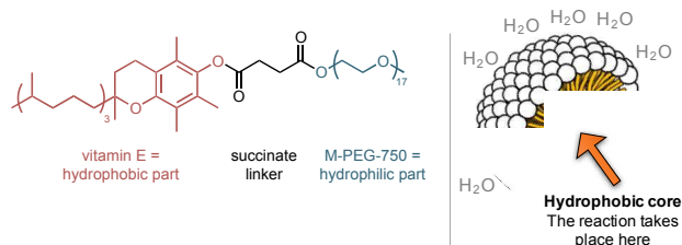
Fig. 1 Structure of TPGS-750-M and micelle formation
