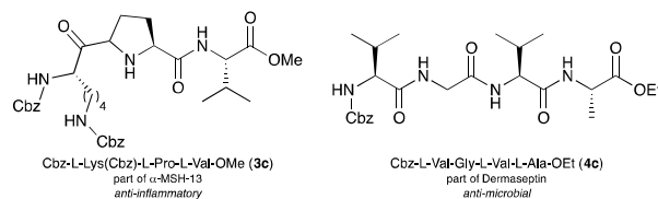
Fig 3 Precursors of biologically active peptides via a 2-step, 1-pot process
