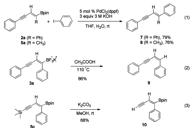
Scheme 2. Derivatization of Boron-Substituted Enynes
