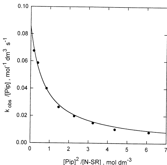
Fig. 1. Dependence of k_{\text{obs}}/[\text{Pip}] on [\text{Pip}]^2/[\text{N-SR}] , ( \text{R} = t\text{-Bu} ) for reaction of 1e with piperidine at 25°C.
