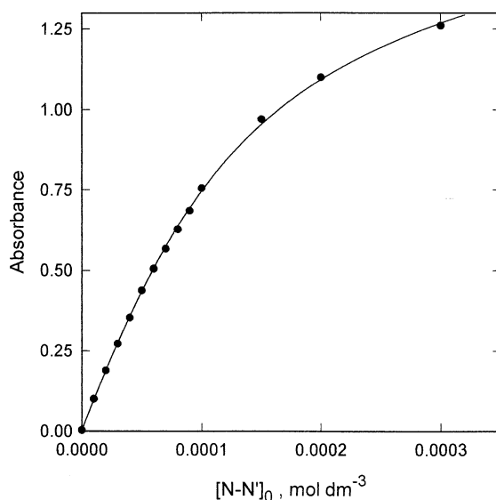
Fig. 2. Fit of absorbance at 400 nm to [\text{N-N}'] for the exchange equilibrium on 1g (Eq. 4; \text{N-N}' = \text{C}_5\text{H}_4\text{N-2-CH=NC}_6\text{H}_4\text{OMe-4} ) in \text{CHCl}_3 at 25^\circ\text{C} .
