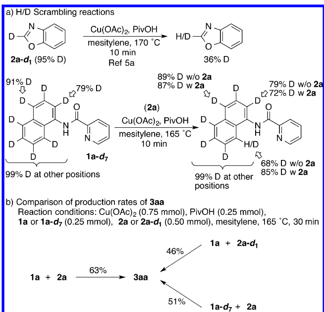
Scheme 3. Deuterium-Labeling Experiments
