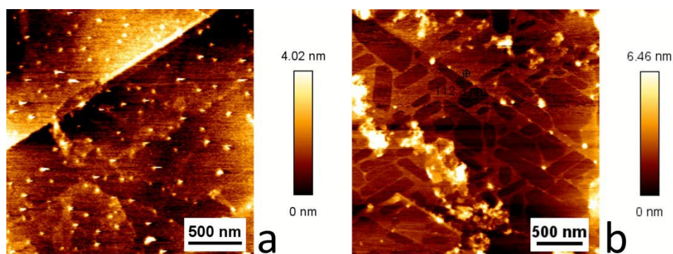
Figure 6. AFM scans of [\text{Cu}(\text{Tp}^{(1\text{Ni})2})(\text{CO})] (a) and [\text{Cu}(\text{Tp}^{(2\text{Ni})2})(\text{CO})] (b) drop casted on HOPG. The domains visible in (b) have lengths and widths of hundreds of nm and a step height of approximately 10 \text{ \AA} corresponding to monolayer coverage.
