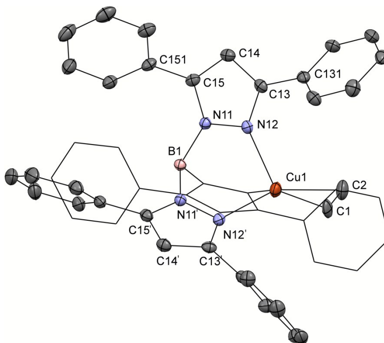
Figure 1. Displacement ellipsoid plot (50% probability level) of [Cu(Tp^{Ph_2})(C_2H_4)] at 110(2) K. Hydrogen atoms have been omitted and one of the arms of the trispyrazolylborate ligand is shown as a wireframe projection for the sake of clarity, only one of the three orientations of the ethene ligand is shown. Symmetry operation ' = [1-y, 2+x-y, z] , symmetry operation for the wireframe segment = [y-x-1, 1-x, z] .
