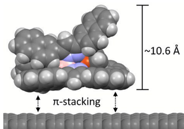
Figure 5. Impression of the proposed stacking of the complex [\text{Cu}(\text{Tp}^{(2\text{Ni})2})(\text{C}_2\text{H}_4)] onto graphene. The X-ray crystal structure of [\text{Cu}(\text{Tp}^{(2\text{Ni})2})(\text{CO})] has not been determined but the compound is assumed to have roughly the same dimensions.
