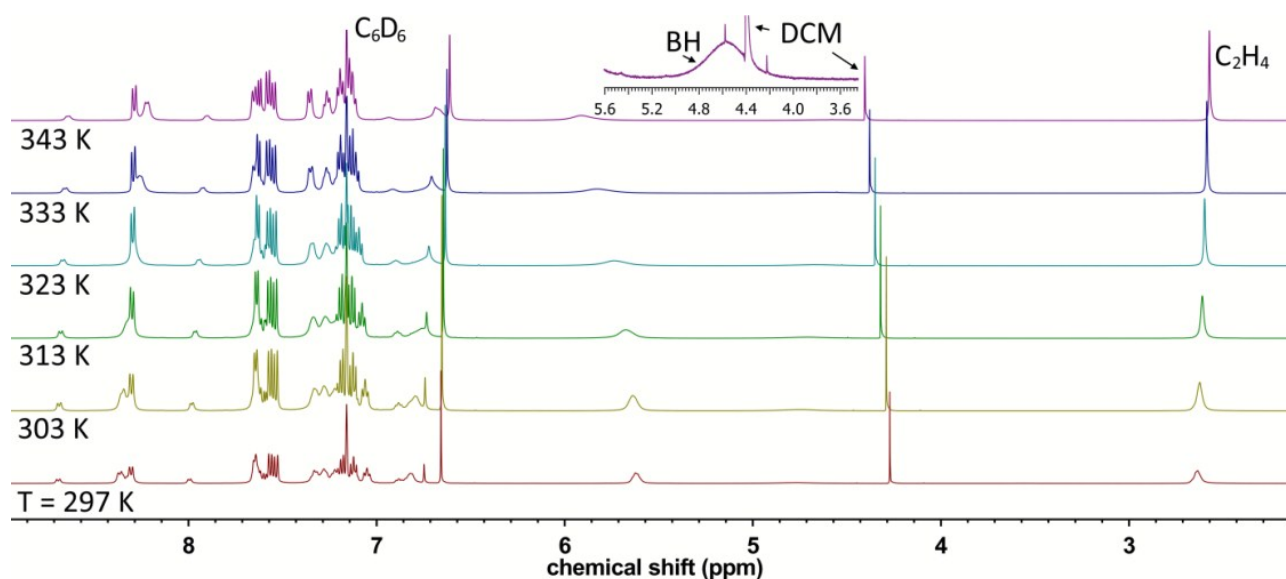
Figure 3. Variable temperature ^1\text{H} -NMR spectra of [\text{Cu}(\text{Tp}^{(1\text{Nt})2})(\text{C}_2\text{H}_4)] in \text{C}_6\text{D}_6 . The inset shows the borohydride peak, the small singlet on top of the \text{BH} peak is a ^{13}\text{C} -satellite peak of the DCM.
