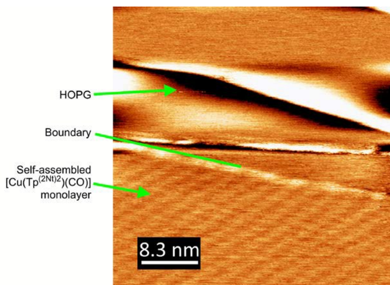
Figure 8. STM scan of [\text{Cu}(\text{Tp}^{(2\text{Nt})_2})(\text{CO})] on HOPG. In the lower half of the image a discrete domain of self-assembled [\text{Cu}(\text{Tp}^{(2\text{Nt})_2})(\text{CO})] is clearly distinguishable from the bare HOPG planes in the top half of the image.
