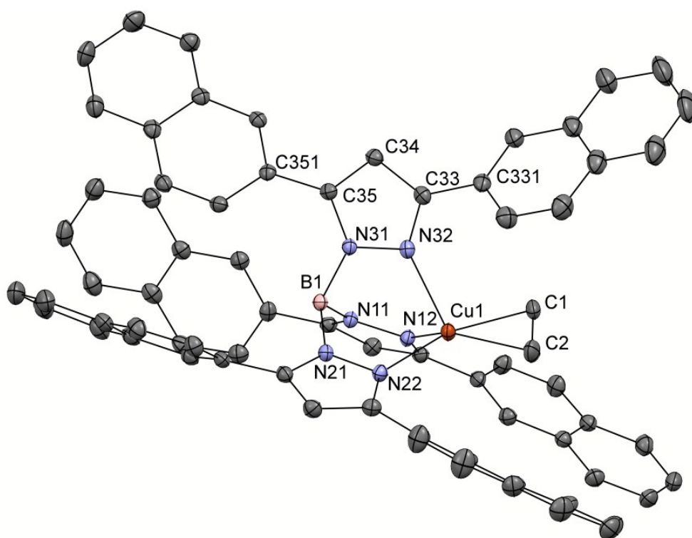
Figure 2. Displacement ellipsoid plot (50% probability level) of one of the independent molecules [\text{Cu}(\text{Tp}^{(2\text{Nt})2})(\text{C}_2\text{H}_4)] at 110(2) K. Hydrogen atoms and solvent molecules were omitted for the sake of clarity.
