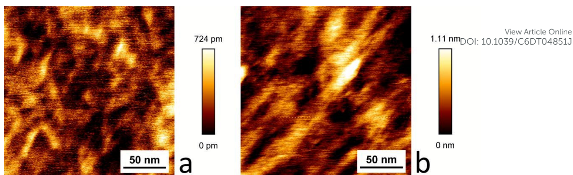
Figure 7. AFM scans of dip-coated samples of [\text{Cu}(\text{Tp}^{(1\text{Nt})2})(\text{CO})] (a) and [\text{Cu}(\text{Tp}^{(2\text{Nt})2})(\text{CO})] (b) on graphene.
