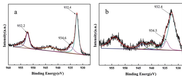
Fig. 6 XPS analysis of virgin catalyst and recycled catalyst.
