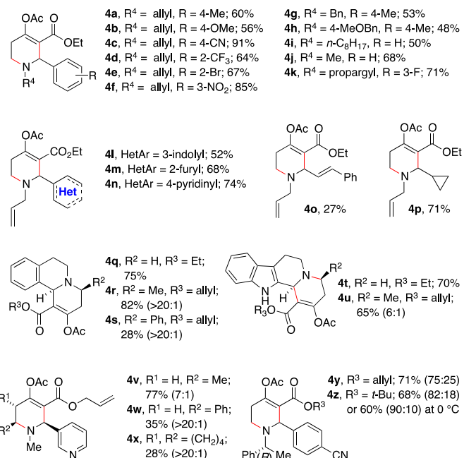
Figure 1. Scope of Two-Step Synthesis of Highly Functionalized Tetrahydropyridines.
