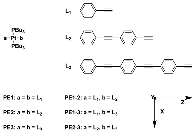
Figure 1. Chemical formulas and nomenclature. Arrows show molecular axes. Nomenclature for the asymmetric compound a-Pt(PBu 3 ) 2 -b , designated as PEa-b , labels two ligands of the compound. In discussions below, ligand a is designated as the “left ligand” and ligand b is the “right ligand”. When a = Cl, the chromophore is designated as “ half-PEb ”. The butadiyne PEn-C≡C-C≡C-PEn is labeled as “ PEn-BD ”.
