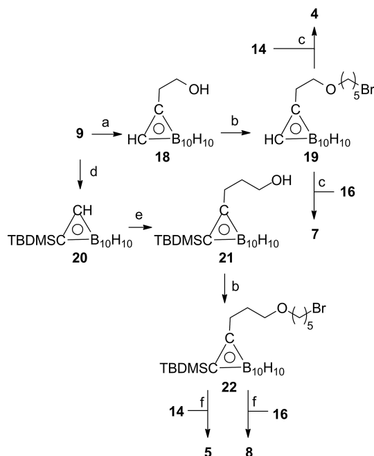
Scheme 2. Reagents and conditions: (a) 1) n BuLi, THF; 2) ethylene oxide (2.5–3.3 M), THF (65%); (b) 1,5-dibromopentane, NaH, TBAI, THF, 0 °C to reflux (79% 19 , 65% 22 ); (c) 1) 14 or 16 , K 2 CO 3 , CH 3 CN, reflux; 2) H 2 (4 bar), Pd/C, 0.01 M HCl (aq), EtOH (3% 4 , 7% 7 ); (d) n BuLi, TBDMSCl, toluene/Et 2 O, 0 °C to room temp. (87%); (e) 1) n BuLi, THF; 2) oxetane, THF (76%); (f) 1) 14 or 16 , K 2 CO 3 , CH 3 CN, reflux; 2) TFA/TBAF, THF, –78 °C to room temp.; 3) H 2 (4 bar), Pd/C, 0.01 M HCl (aq), EtOH (18% 5 , 17% 8 ).
