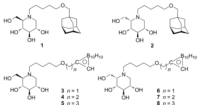
Figure 1. Lead structures AMP-DNM 1 and ido -AMP-DNM 2 and ortho -carborane-substituted analogues 3–8 subject of the here-presented studies.
