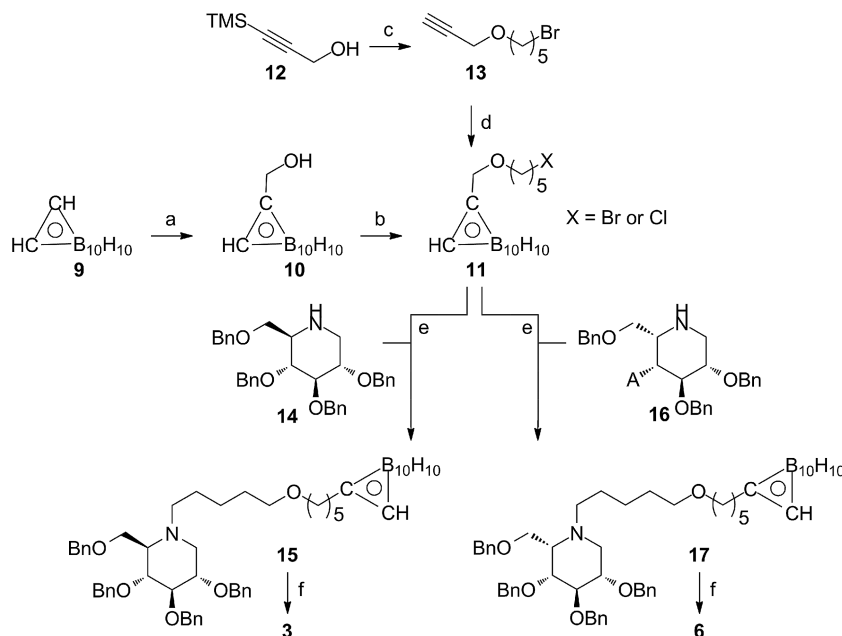
Scheme 1. Reagents and conditions: (a) TBAF, formaldehyde (37% v/v in H 2 O), THF (86%); (b) 1,5-dibromopentane, NaH, TBAI, THF, 0 °C to reflux (9%); (c) NaH, 1,5-dibromopentane, TBAI, THF, 0 °C to room temp. (58%); (d) decaborane, BmimCl, toluene, 80 °C to 105 °C (62%); (e) 14 or 16 , K 2 CO 3 , CH 3 CN, reflux ( 15 : 59%, 17 : 78%); (f) H 2 (4 bar), Pd/C, 0.01 M HCl (aq), EtOH ( 3 : 13%, 6 : 19%).
