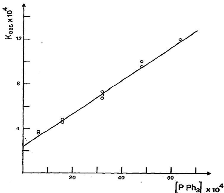
Fig. 2. Plot of k_{obs} (s^{-1}) vs. [PPh_3] (X10^4 M) for the reaction of resin R_1 with PPh_3 .
